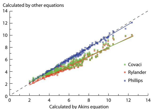
Figure 4-10. Calculation of total lipids in serum from enzymatic data.
