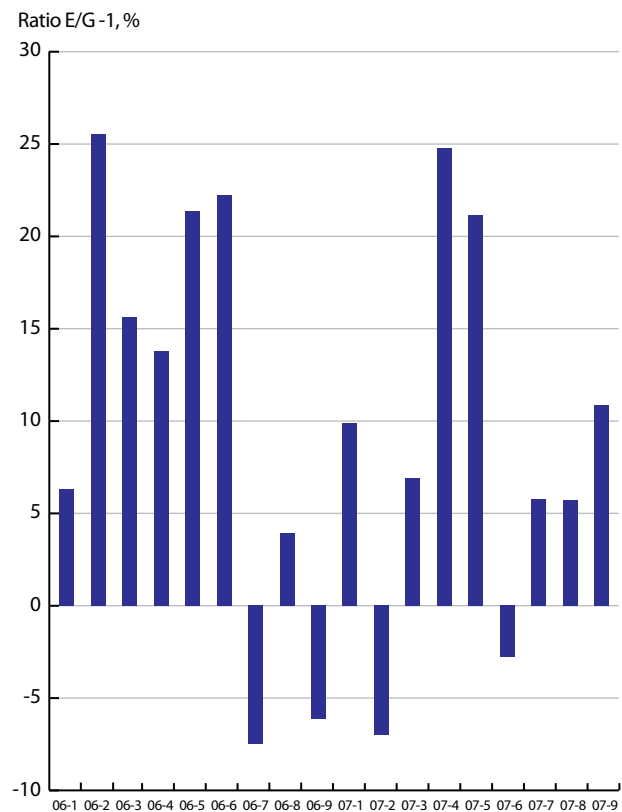
Figure 4.9. Comparison of total lipid results obtained from gravimetric and enzymatic methods.
