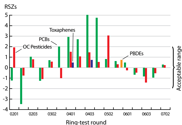
Figure 4.5. An individual participant's performance using RSZs.
