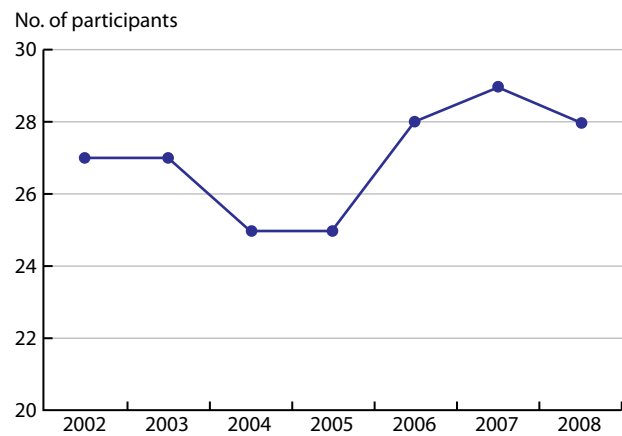
Figure 4.2. Trend in participation in the AMAP Ring-tests.
