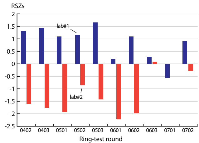
Figure 4.8. A comparison of lipid results for two laboratories.
