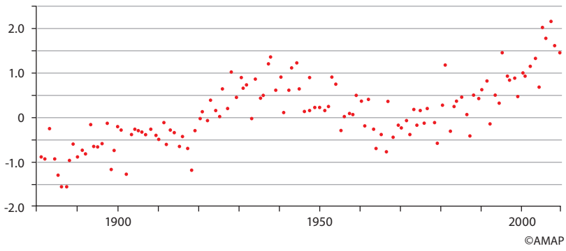
Temperature change relative to the 1961–1990 mean, °C
