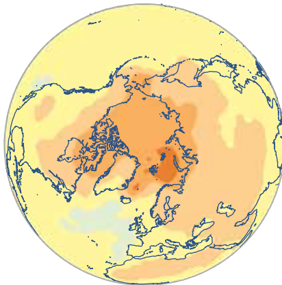
Hindcast 50-year change in temperature (1957–2006) based on a number of IPCC climate models
