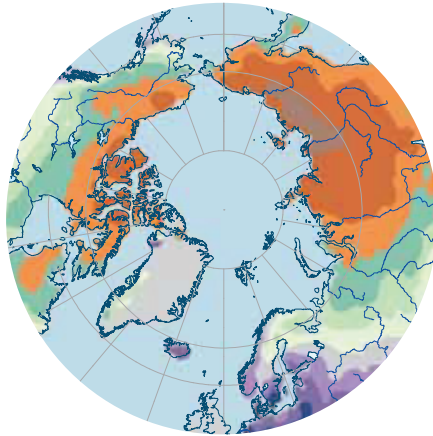
Projected change in mean monthly SWEmax from 1970-1999 to 2049-2060, %
