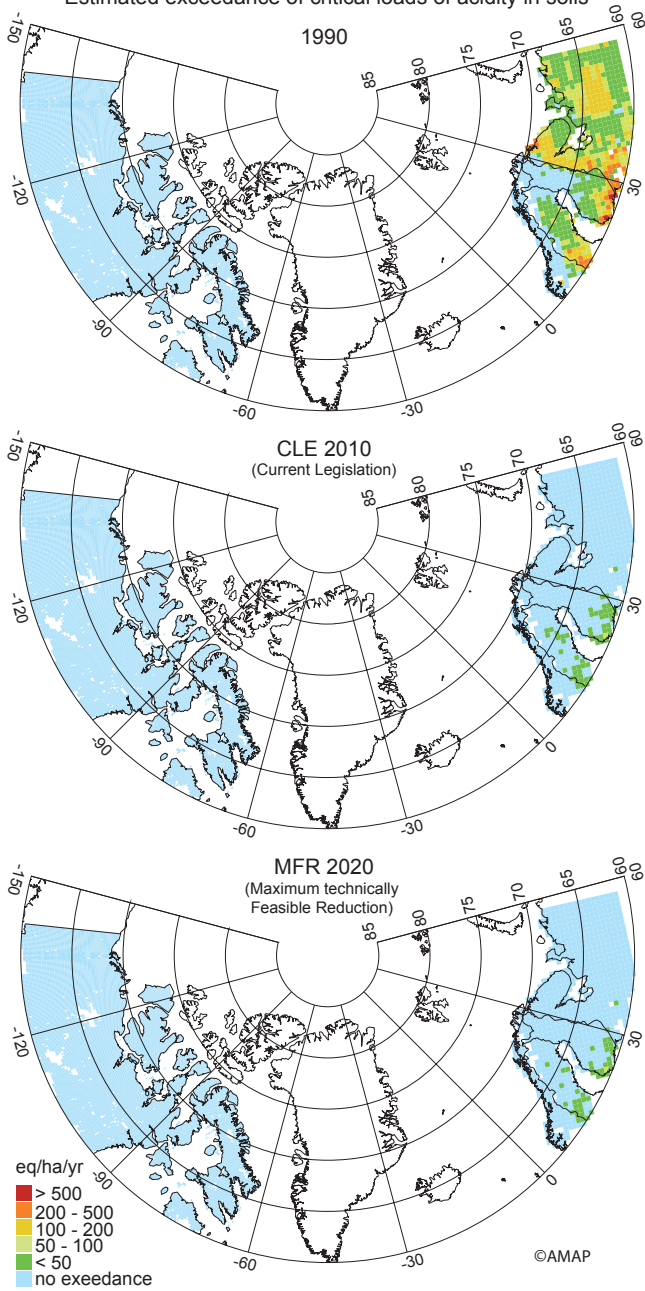
Estimated exceedance of critical loads of acidity in soils
