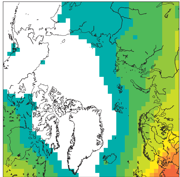
NO 3 concentration in 2000, µg/m 3
