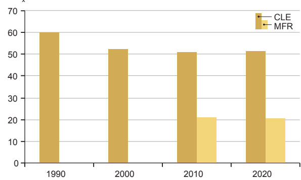
SO x -S emissions, Mt
