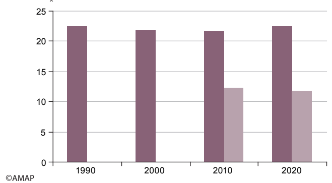
NO x -N emissions, Mt
