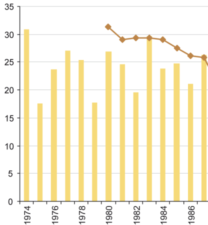
SO 2 concentrations in air at Svanvik, µg/m 3
