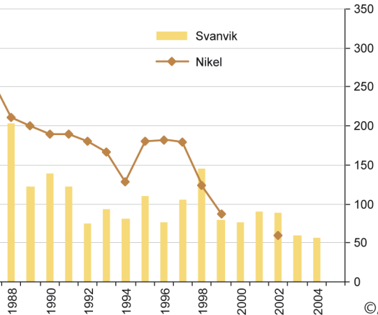
SO 2 emissions from Nikel, kt
