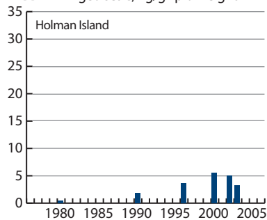
ΣPBDE in seabird eggs, ng/g lipid weight
