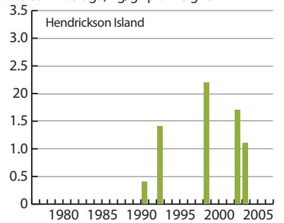
ΣPBDE in ringed seals, ng/g lipid weight
