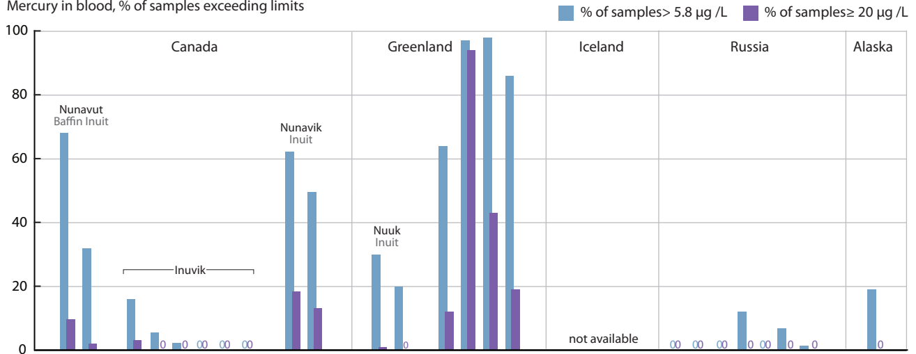
Mercury in blood, % of samples exceeding limits
